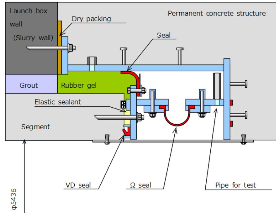
11. Overview design
