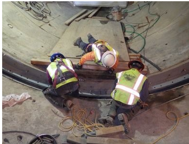
5. Installation of bolts
