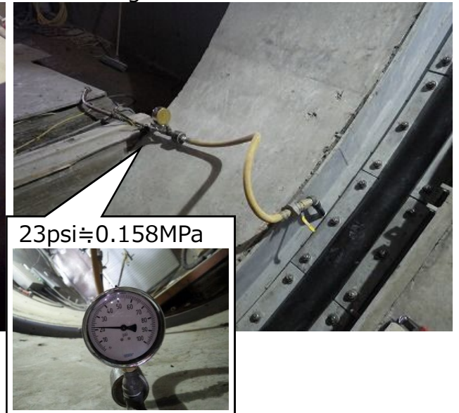
9. Watertightness test at site
